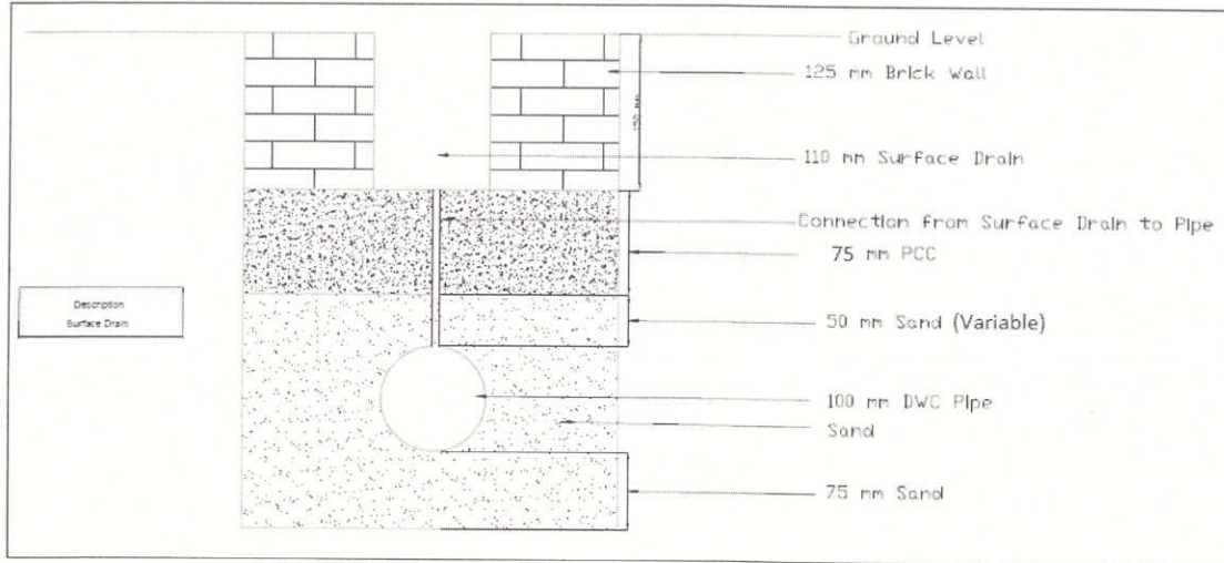
SECTIONAL VIEW- Surface Drain & DWC Pipe
